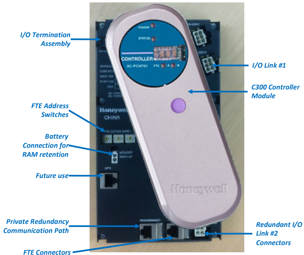
Figure 1 - C300 Controller
