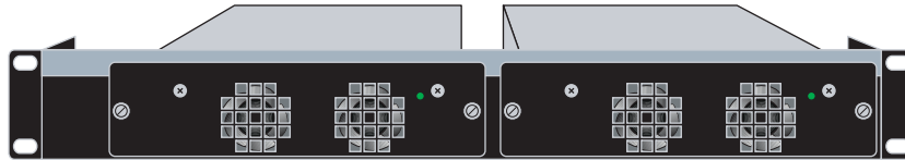
Figure 3. Redundant Power Supply Chassis (P0973BN) - Two Slot
